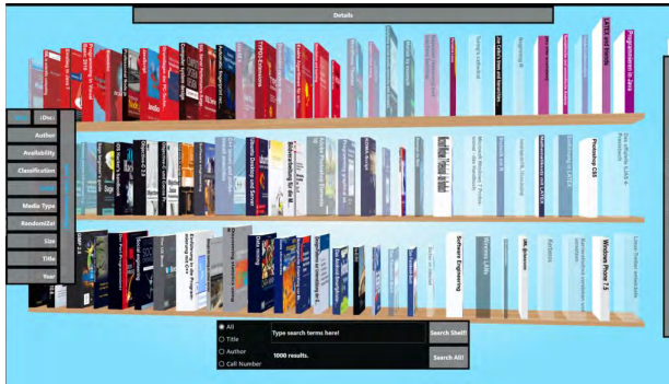
Blended Shelf
