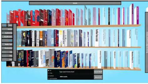
Blended Shelf
