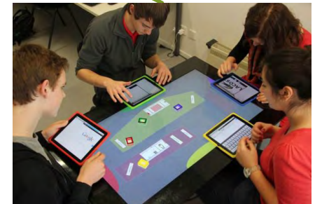
Twister Search
