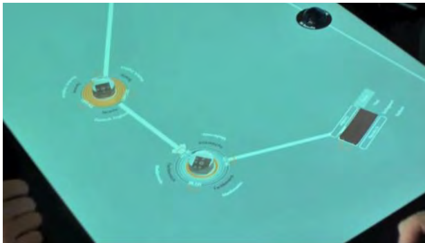
FacetSearch++
