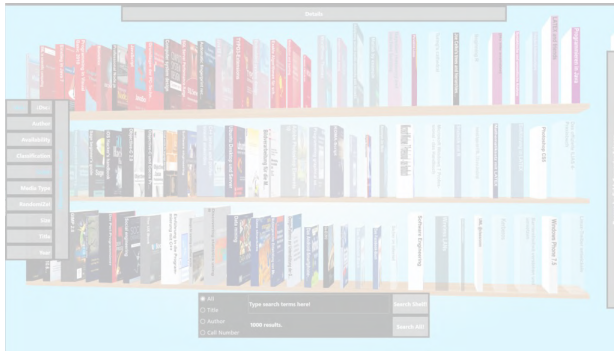
Blended Shelf
