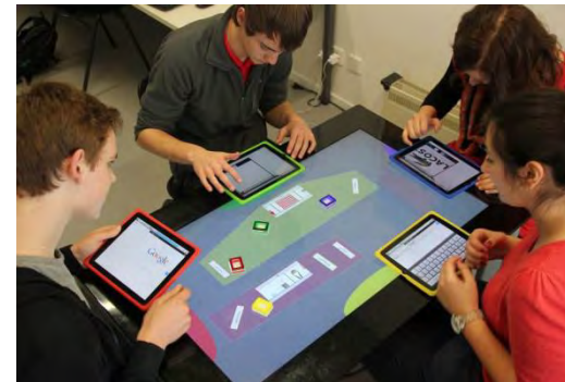
Twister Search
