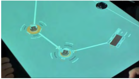
FacetSearch++
